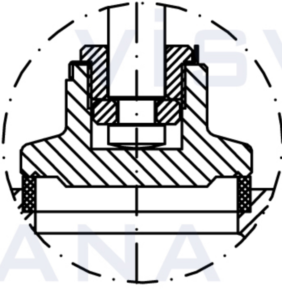
DN 15...DN 80
