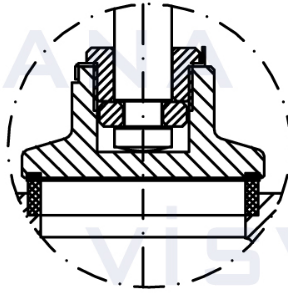
DN 100...DN 350
