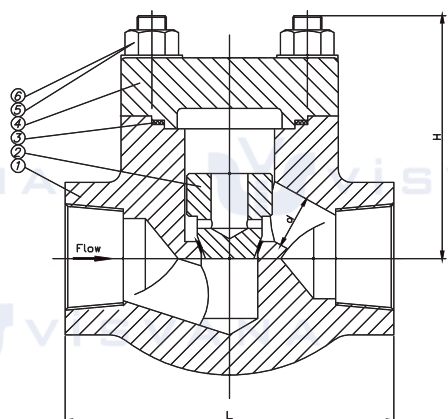
Lift Check Valve
