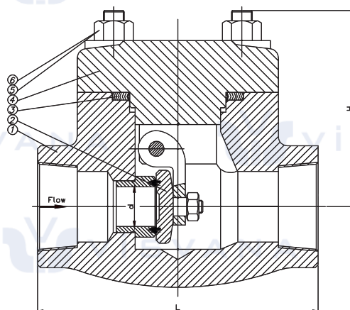
Swing Check Valve
