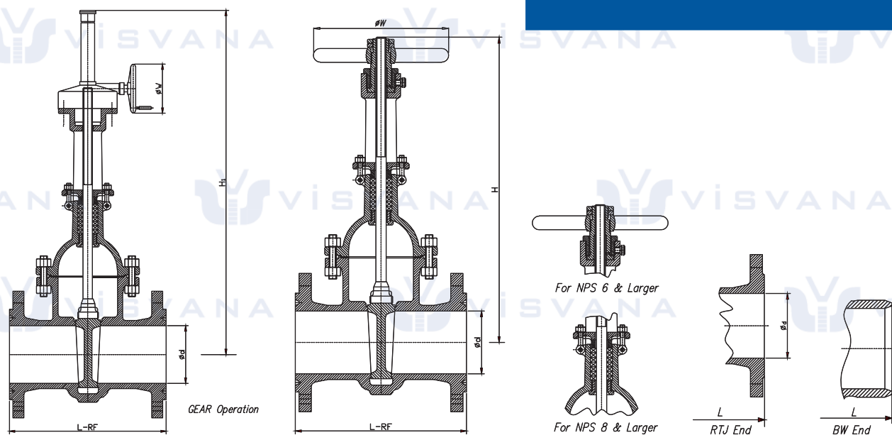
Class 600 &amp; Class 900 Gate Valve
